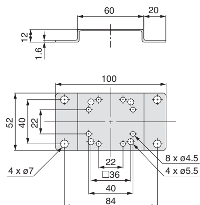
Fixation plate
