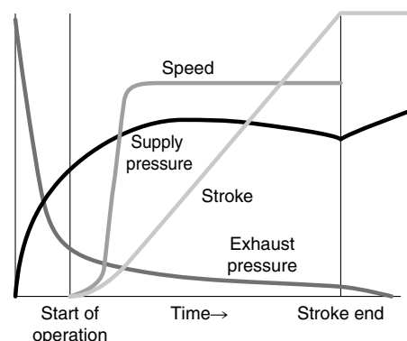
Feature of meter-in control
