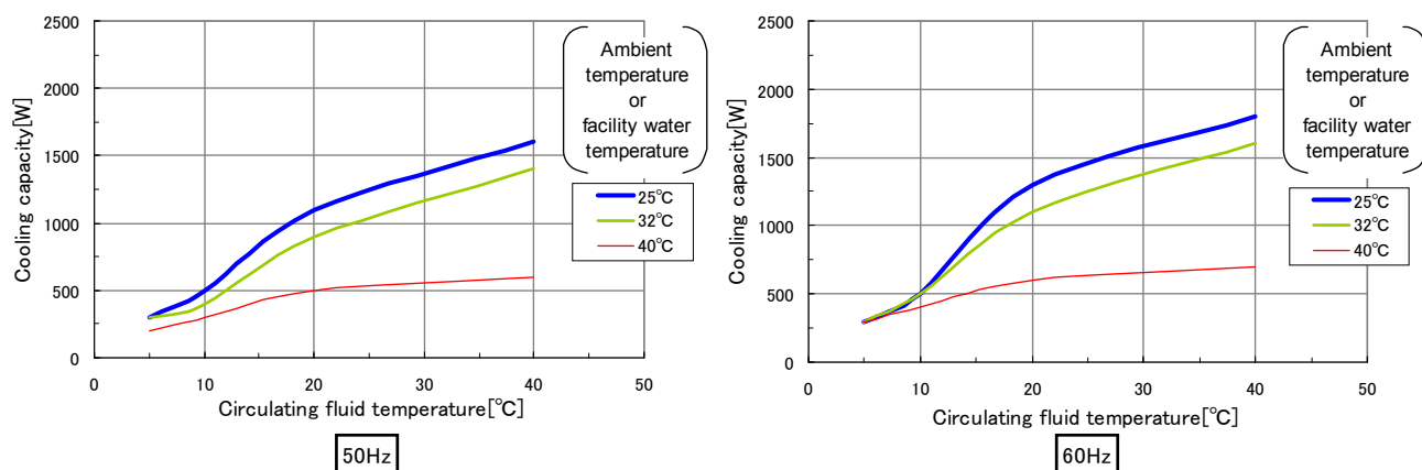
Fig. 9-6 Cooling capacity(HRS012-**-20)
