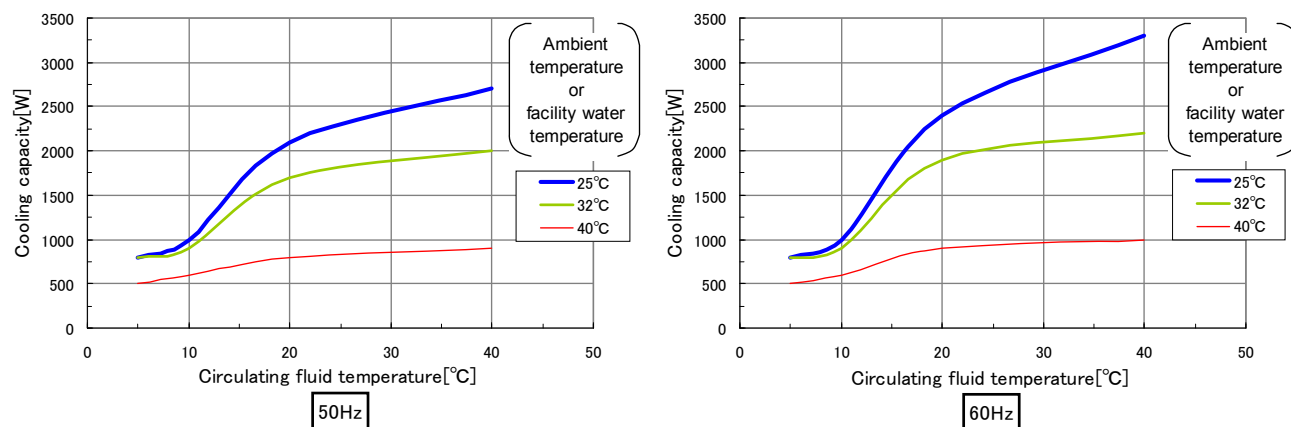
Fig. 9-8 Cooling capacity (HRS024-**-20)
