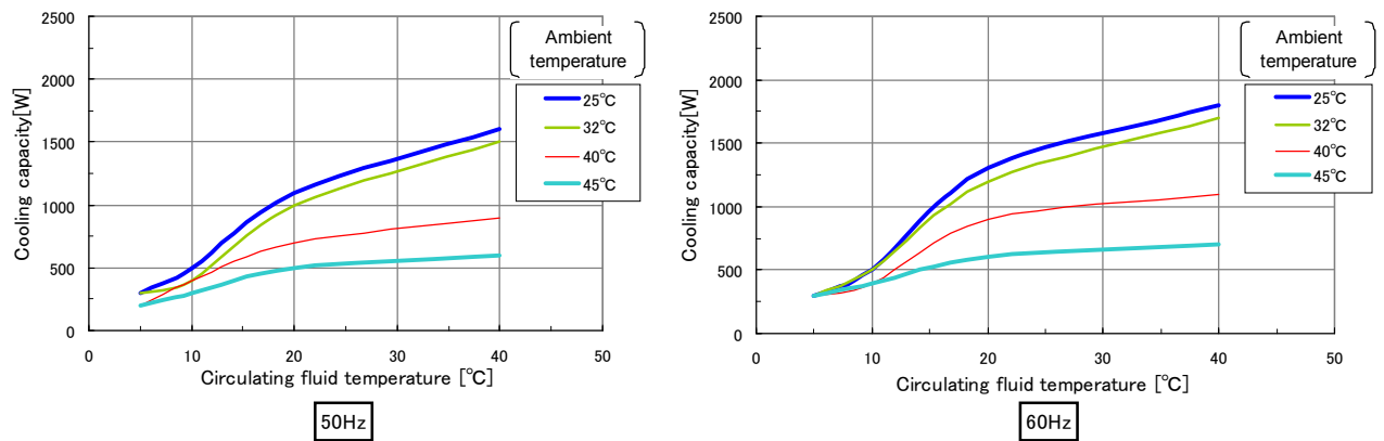
Fig. 9-9 Cooling capacity (HRS012-A*-20-G)
