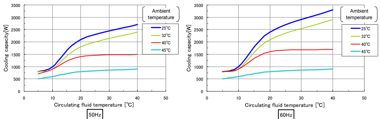
Fig. 9-11 Cooling capacity (HRS024-A*-20-G)
