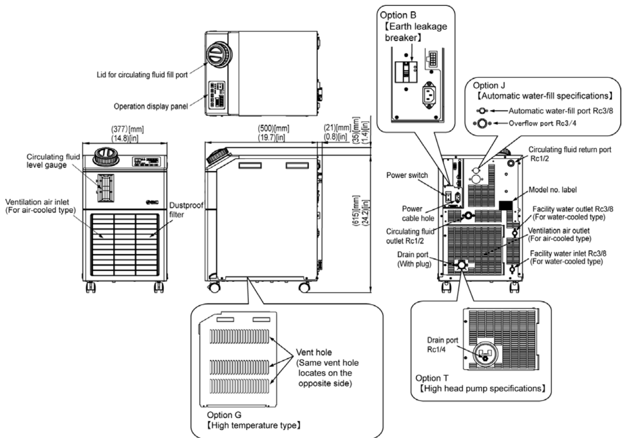
Fig. 9-1 Outline dimensions
