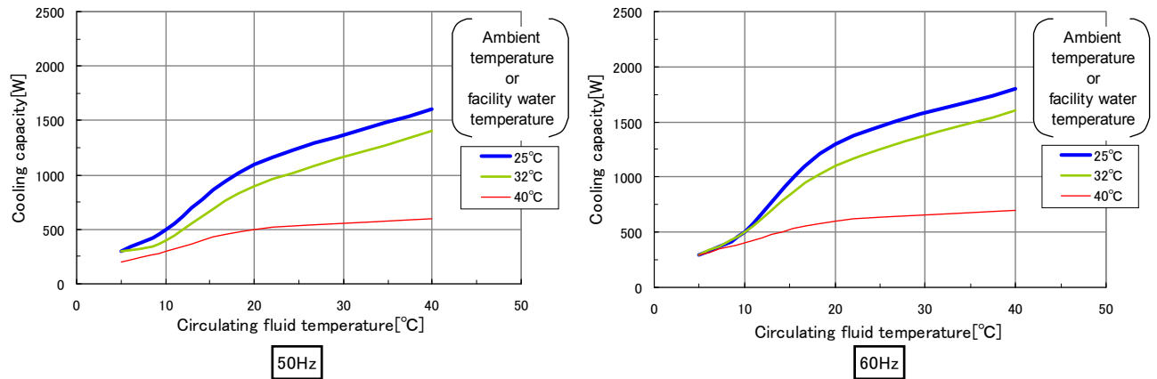
Fig. 9-4 Cooling capacity(HRS012-**-10)
