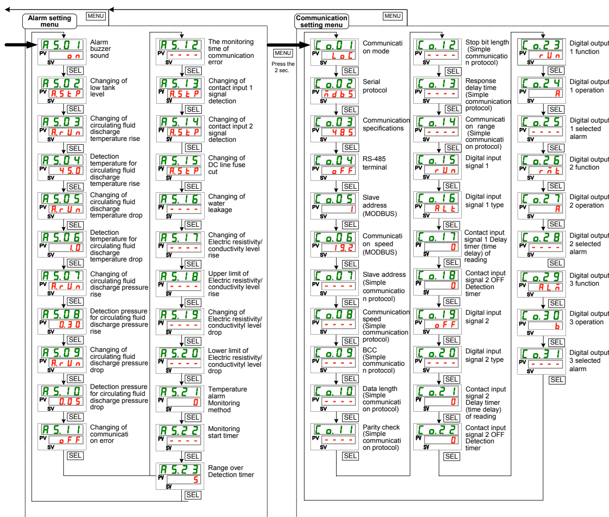
Fig. 5.2-2 Key operation (2/2)
