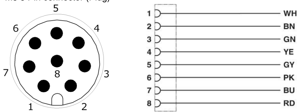
M8 8 Pin connector (Plug)
