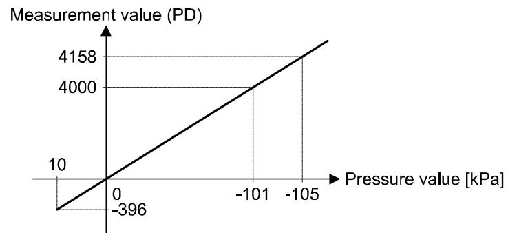
Relationship between the measurement value (PD) and pressure value (Range: -101 kPa, Unit: kPa)
