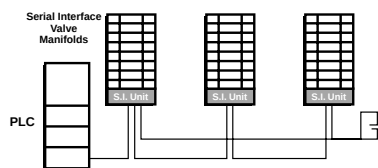
SERIAL INTERFACE Control System
