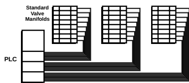
HARD-WIRED Control System
