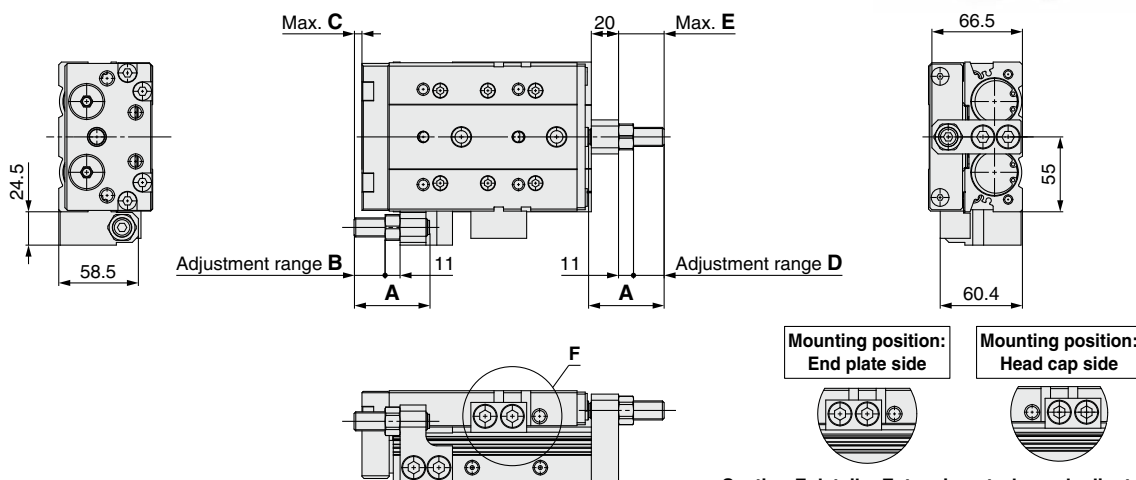
Section F details: Extension stroke end adjustment block mounting position
