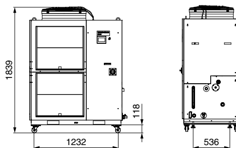
Fig. 1 Mounting view
