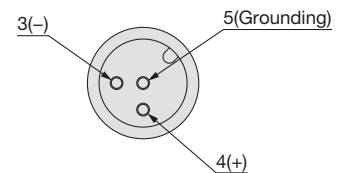
Details of manual override part (for manual operation) Type E
