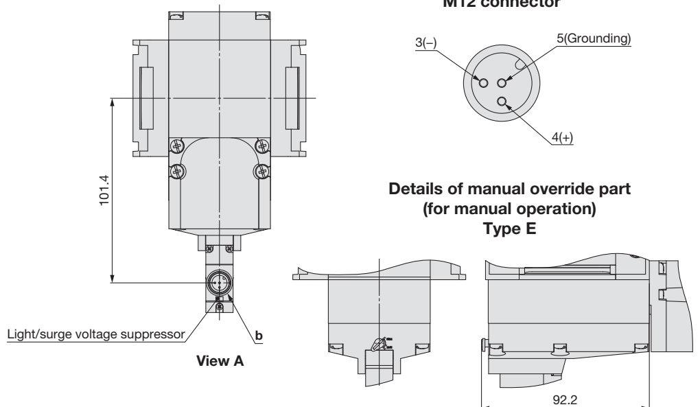
Detailed figure of b section M12 connector
