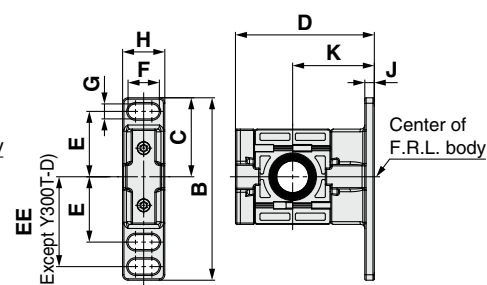
Spacer with bracket (Standard)
