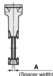
Spacer with bracket (Long type)
