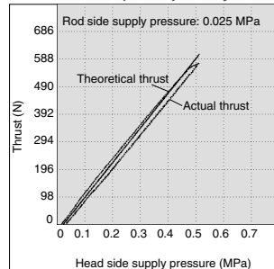
CQ2XB40-75D (Low speed cylinder)
