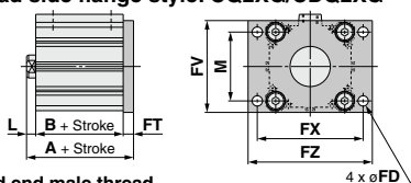
Rod end male thread
