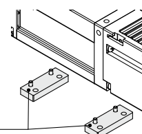
Adapter assembly for bottom mounting
