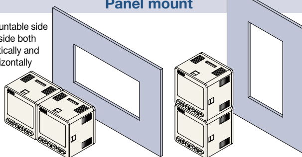
Panel mount
