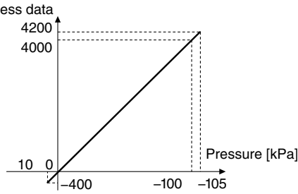
PSE541-L (For negative pressure)
