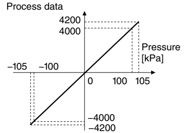
PSE543-L (For compound pressure)
