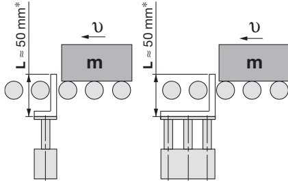
MGPKFM6 to 25 (Slide bearing)
