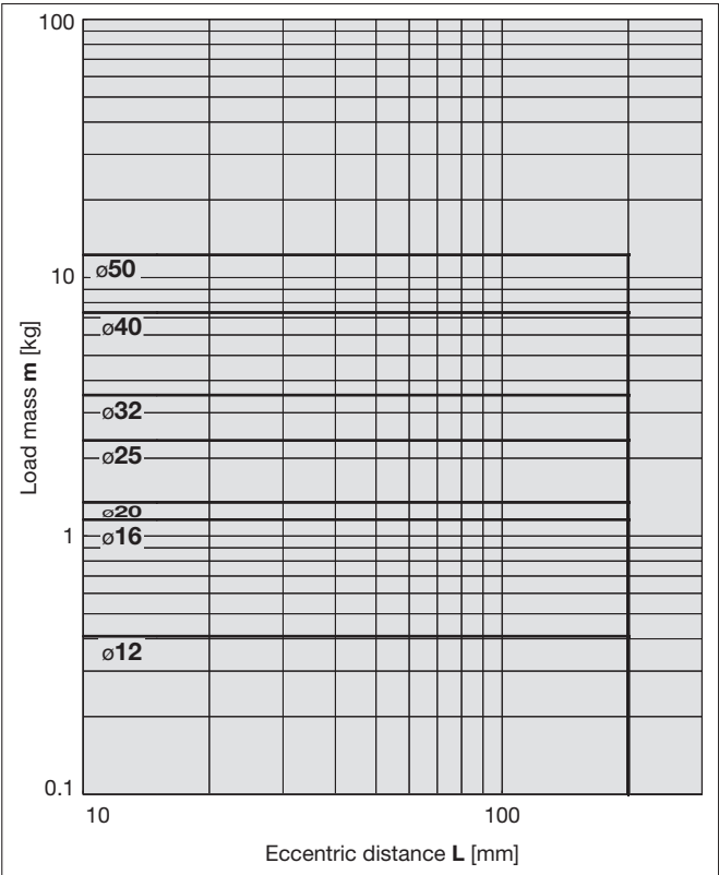
8 Over 100 mm stroke, V = 400mm/s
