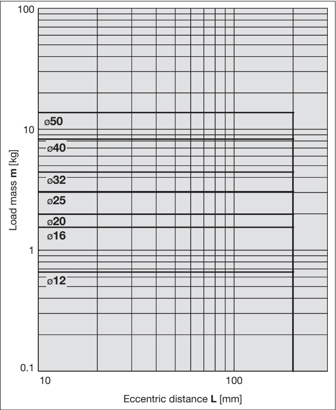
6 Over 30 mm stroke and 50 mm stroke or less, V = 400mm/s
