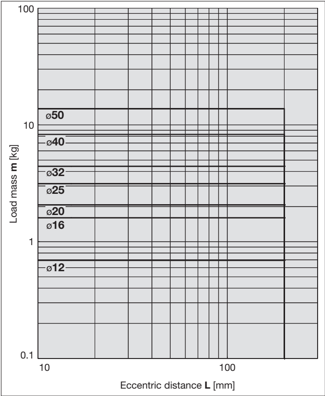
5 30 mm stroke or less, V = 400mm/s
