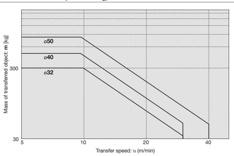
MGPKSFM32 to 50 (Slide bearing)
