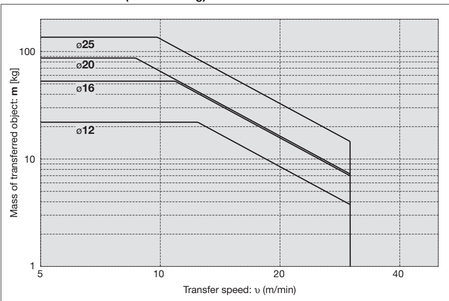
MGPKSFM12 to 25 (Slide bearing)
