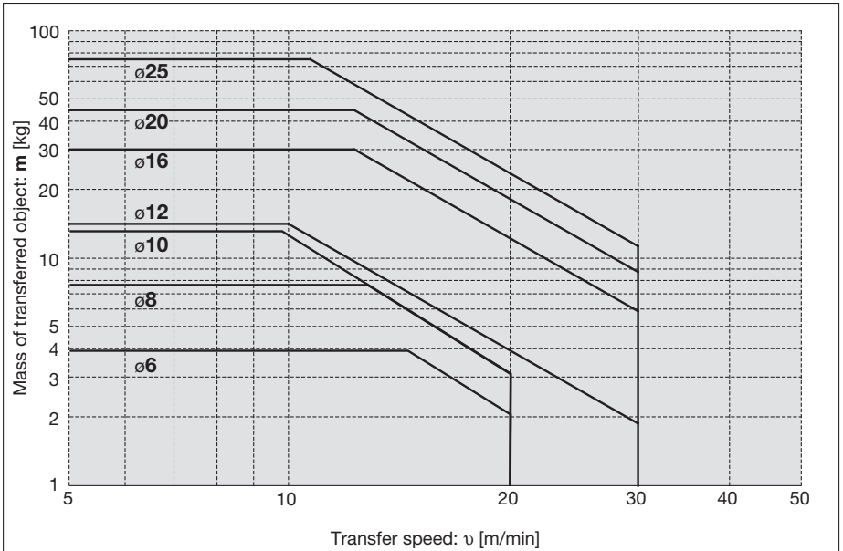
MGPKFM6 to 25 (Slide bearing)
