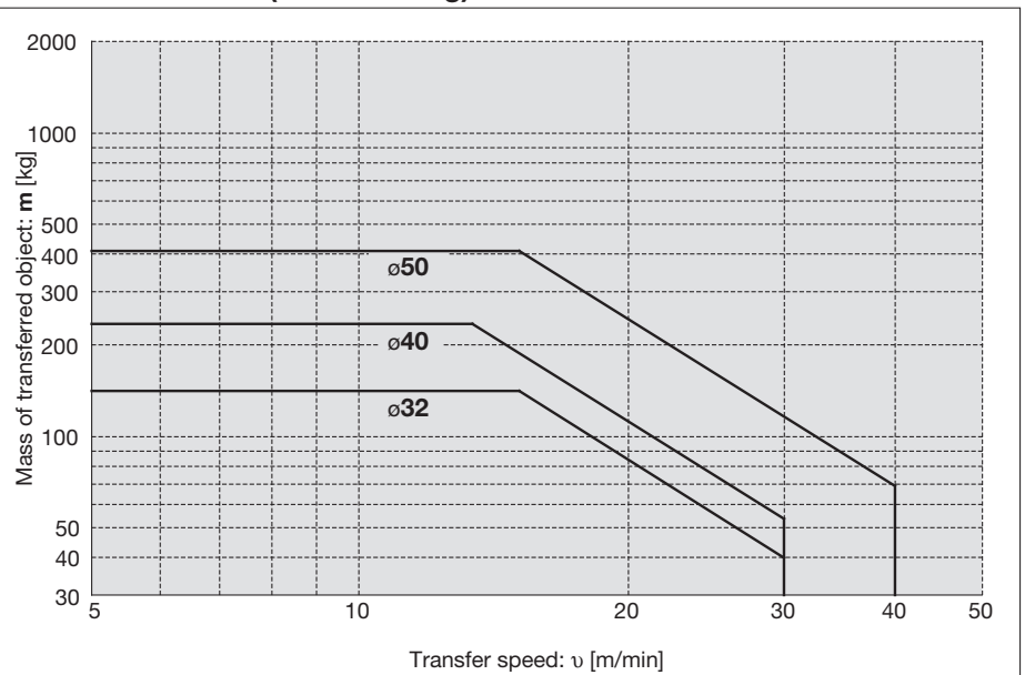
MGPKFM32 to 50 (Slide bearing)
