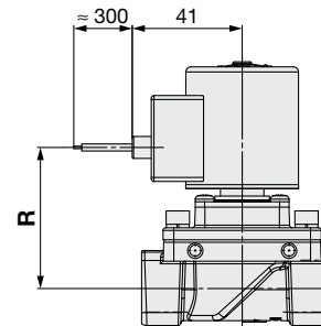
GS: Grommet with PCB
