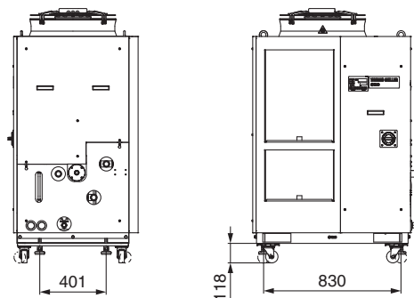
Fig. 1 Mounting view
