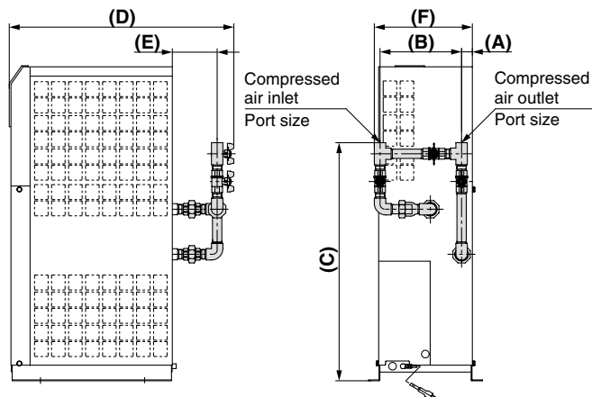
Dimensions (mm)
