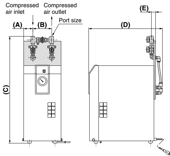
Dimensions (mm)
