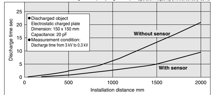
Installation distance and discharge time (Air purge: Yes)
