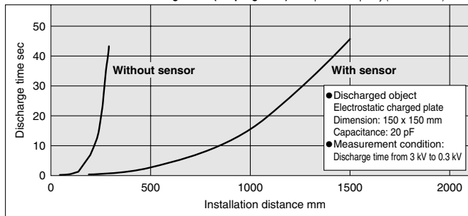
Installation distance and discharge time (Air purge: No)
