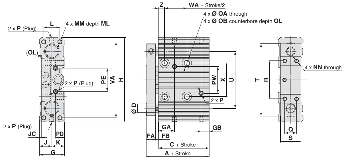
Bottom view
