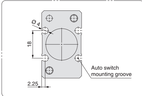
Dimensions of auto switch mounting groove
