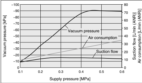
Nominal Nozzle Size \phi 0.7 Specification: Exhaust Characteristics
