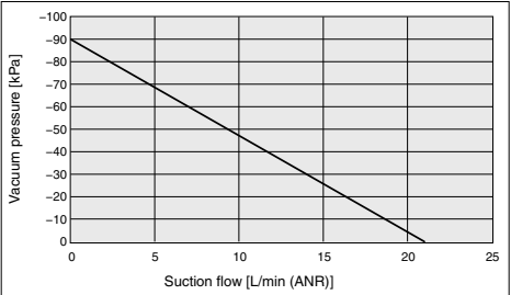
Nominal Nozzle Size \phi 1.0 Specification: Flow Rate Characteristics
