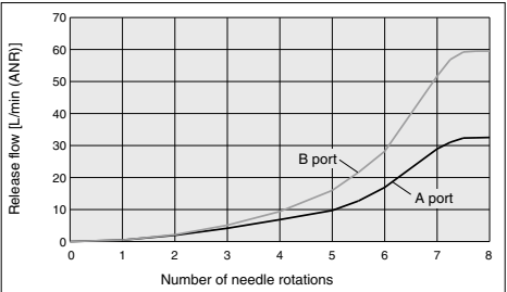
Nominal Nozzle Size \phi 1.0 Specification
