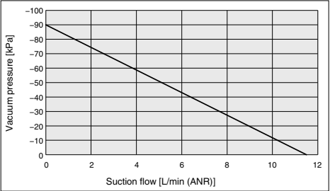
Nominal Nozzle Size \phi 0.7 Specification: Flow Rate Characteristics
