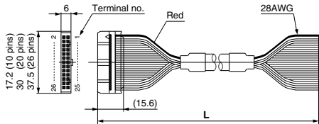
Flat ribbon cable connector
