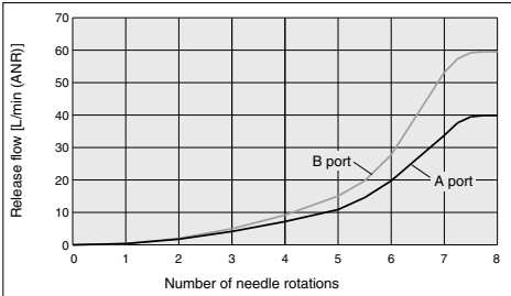
Nominal Nozzle Size \phi 0.7 Specification
