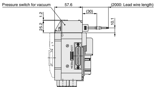
With pressure switch
