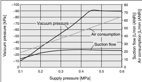
Nominal Nozzle Size \phi 1.0 Specification: Exhaust Characteristics
