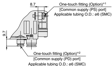
PS and PD port dimensions
