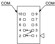
(PH, PHC: 10 pins)
