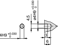
Section C detail (Scale: 2/1)
