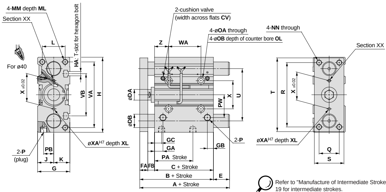
MGPM, MGPL Common dimensions
