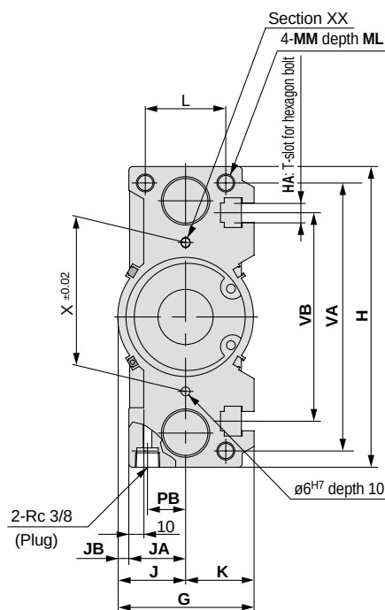
MGPM, MGPL Common dimensions
