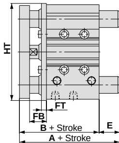
MGPM, MGPL Common dimensions (mm)
