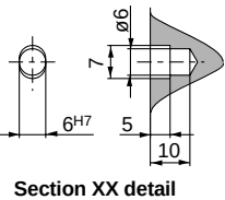
Section XX detail
