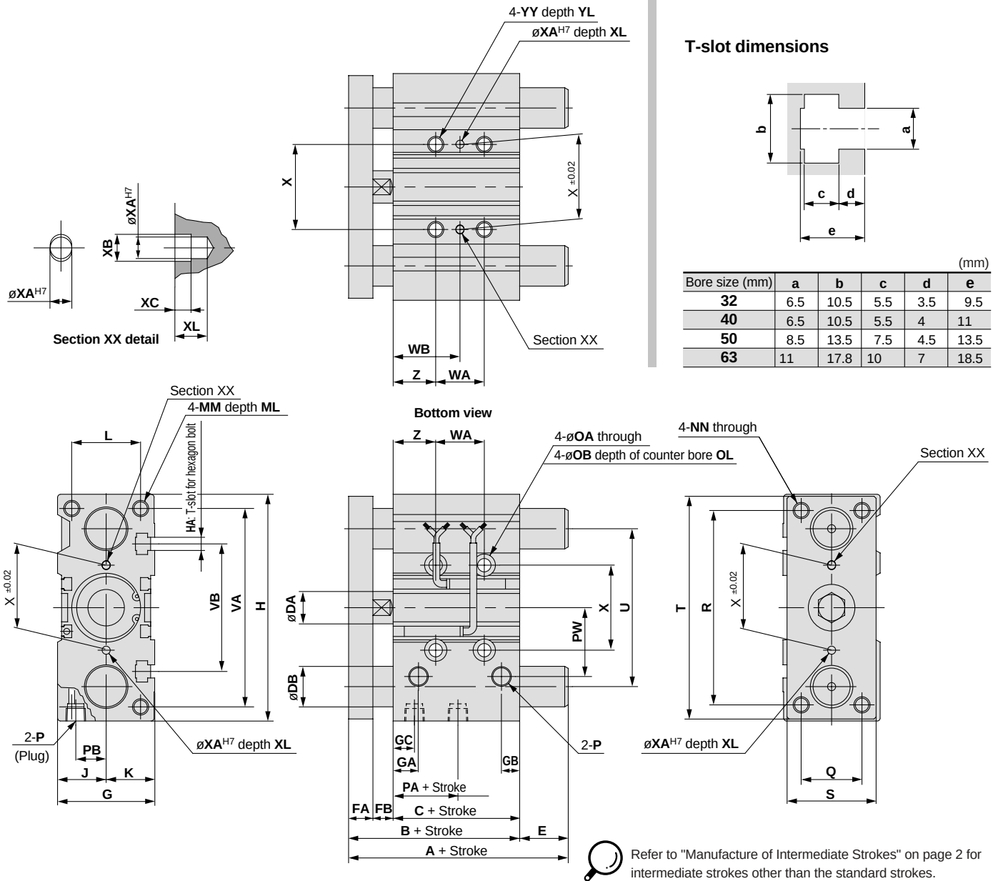
MGPM, MGPL Common dimensions
