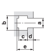
T-slot dimensions [mm]
