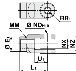
Double knuckle joint
