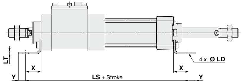
With Rubber Bumper [mm]
