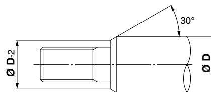
For male thread
