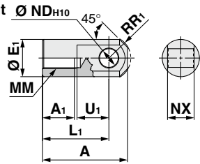
Single knuckle joint Ø ND H10
