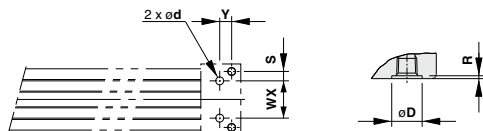
Bottom ported (ZZ) (Applicable O-ring)
