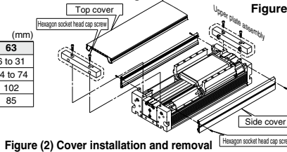
Figure (2) Cover installation and removal
