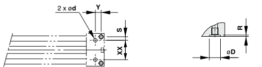
Bottom ported (Applicable O-ring)
