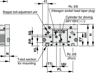
Dimensions of T-slot for mounting
