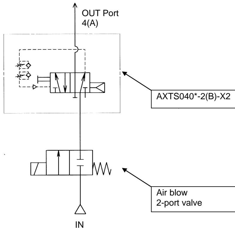
Fig.3 Symbol for internal pilot fluid passage.
