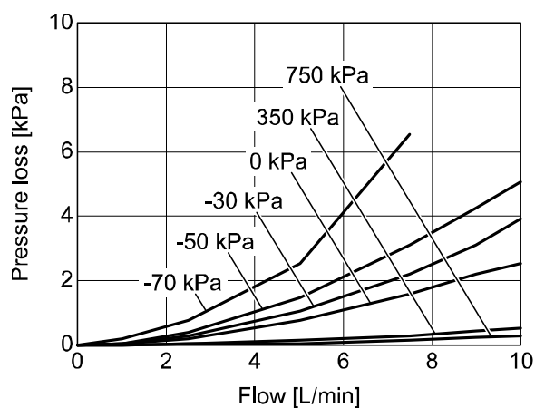
PF2M710 (10 L/min)
