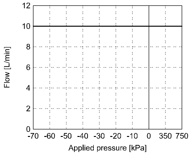
PF2M710 (10 L/min)
