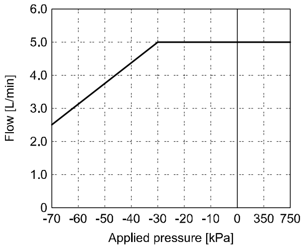
PF2M705 (5 L/min)
