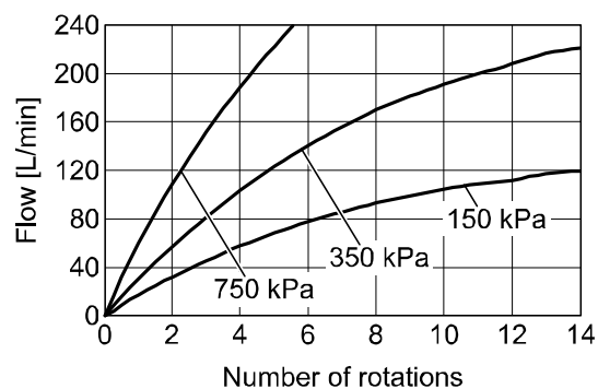
PF2M721 (200 L/min)
