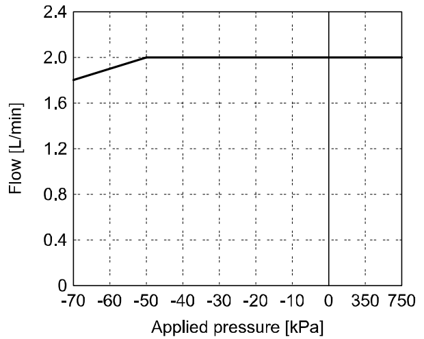
PF2M702 (2 L/min)
