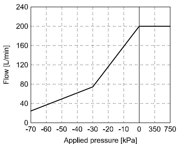
PF2M721 (200 L/min)
