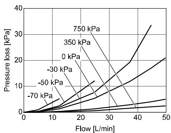
PF2M750 (50 L/min)
