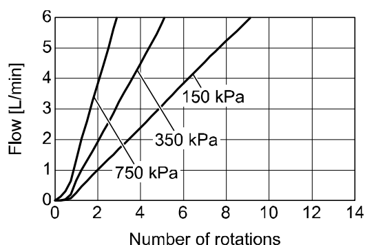
PF2M705 (5 L/min)
