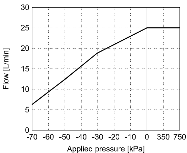
PF2M725 (25 L/min)
