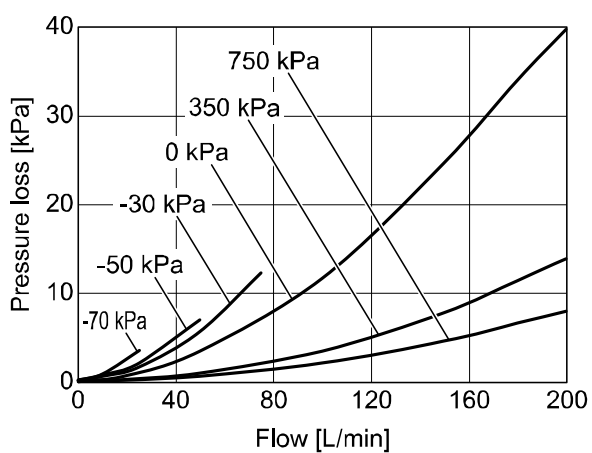
PF2M721 (200 L/min)
