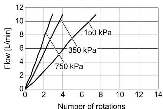
PF2M710 (10 L/min)
