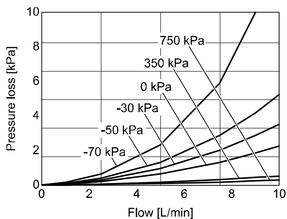
PF2M702 (2 L/min)
