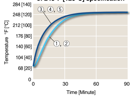
Temperature distribution of 248°F [120°C] specification
