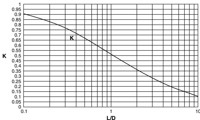
Graph 1. Clausing factor
