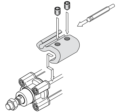
• Mounting example for D-A9□(V),
