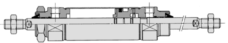
Series CM2W
