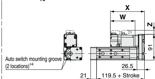
Motor mounting position: Right side parallel LESYH16R S2 T6 □-□
