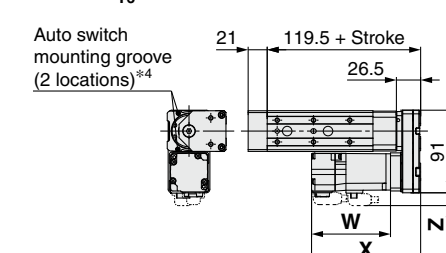
Motor mounting position: Left side parallel LESYH16L S2 T6 □-□
