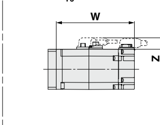
Motor option: With lock LESYH16m S2 T6 □-□B
