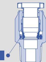
Male connector
