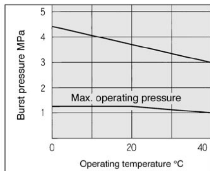
Burst Pressure Characteristics and Operating Pressure Curve
