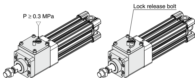
a) Lock released by air pressure
