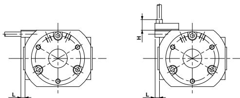
When auto switch D-M9NV, D-M9PV, D-M9BV is used
