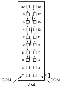
J kit Flat ribbon cable connector (20P) PC wiring system compatible
