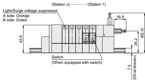
Internal Pilot Manifold L Dimension n: Stations
