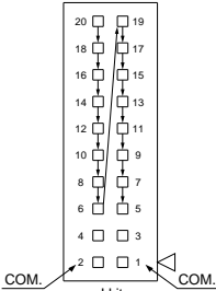
J kit Flat ribbon cable connector (20P) PC wiring system compatible
