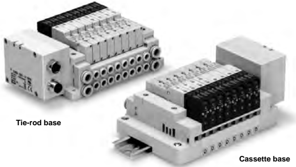
Cassette base
