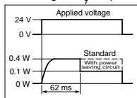
(The electric wave form of the energy saving 10-SYJ5□□0T)
