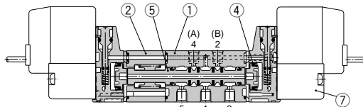
(This figure shows a closed center type.)
