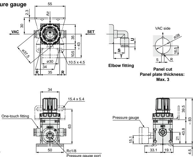
Fitting Part Dimensions (mm)
