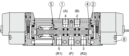
(This figure shows a closed center type.)
