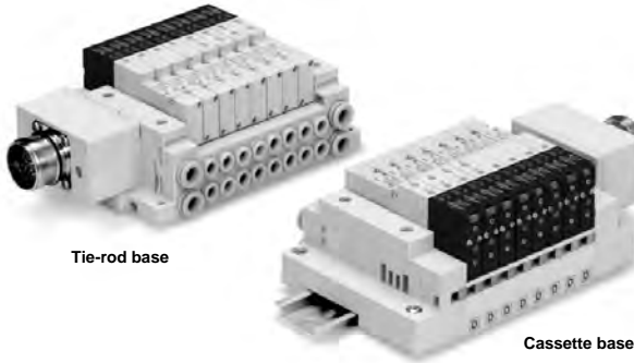
Cassette base
