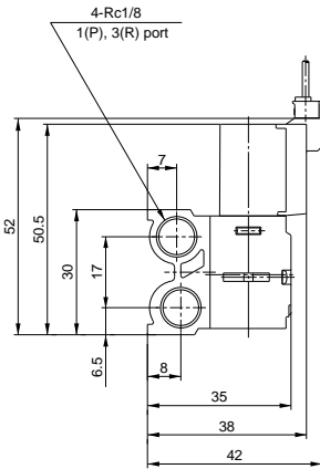
M plug connector (M)
