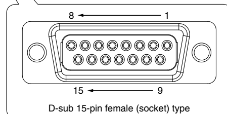
Contact input/output signal connector
