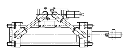
Reverse valve direction/ Rod retracted when energized
