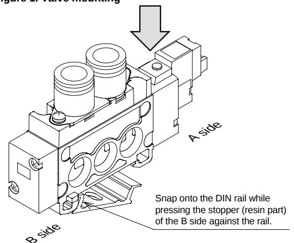
Figure 1. Valve mounting
