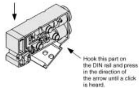
Figure 1. Block mounting
