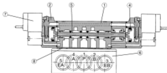
3 position closed centre/exhaust centre/pressure centre
