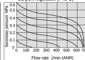
ARBY5000 A1 port regulated (P to A), B1 port regulated (P to B)
