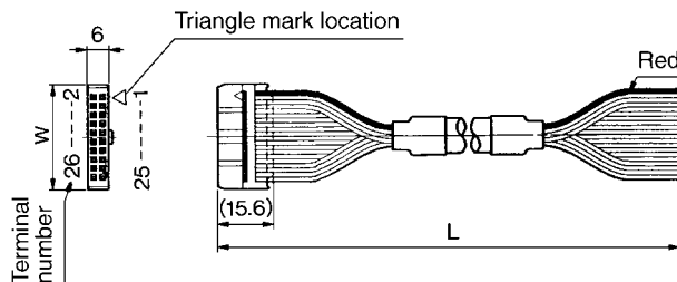
Flat ribbon cable assembly
