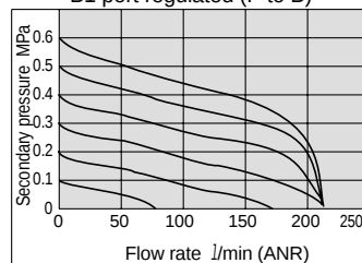
ARBY3000 A1 port regulated (P to A), B1 port regulated (P to B)
