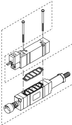
ARBY5000-00-□-2 ARBY7000-00-□-2
