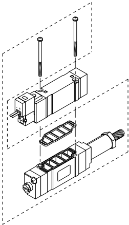
ARBY5000-M1-□-2 ARBY7000-M1-□-2
