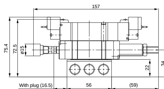
With interface regulator
