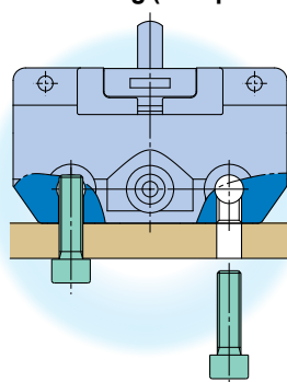
Panel mounting
