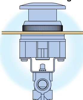
Panel mounting
