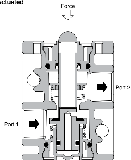
Actuated
