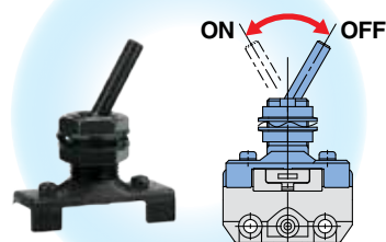
Toggle lever *
