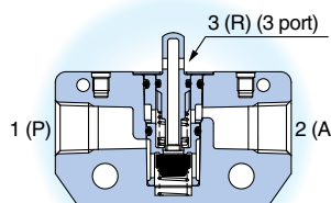
Side ported
