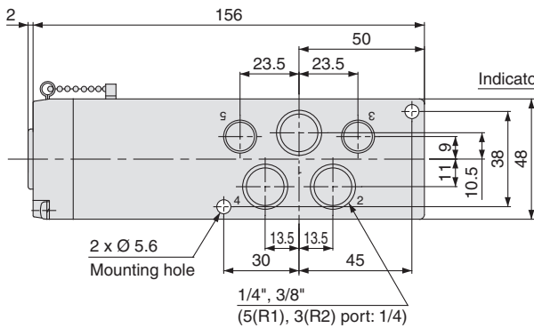
Bottom ported drawing
