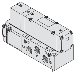
External pilot port 1/8 <Sub-plate>
