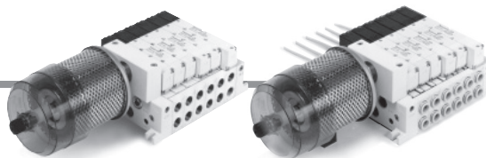
Applicable exhaust cleaner AMC610-10 (Port size Rc 1)
