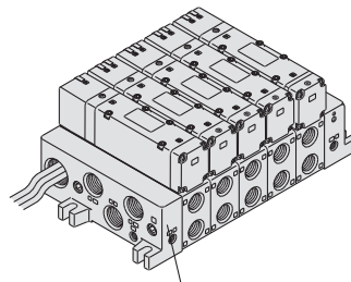
External pilot port 2 x 1/8 <Manifold>
