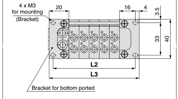
Bracket option: F2 (For bottom ported)
