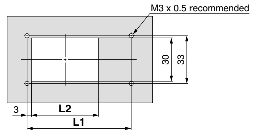
Panel fitting dimensions/Mounting hole dimensions
