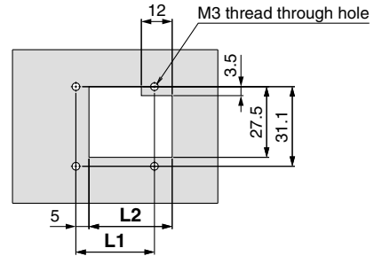
Panel fitting dimensions/Mounting hole dimensions
