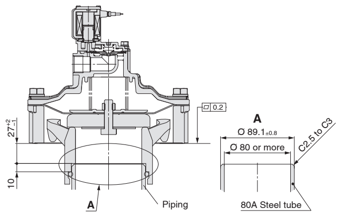
VXF26D□□□□ Piping
