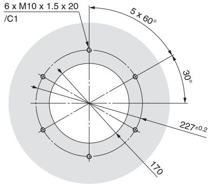
VXF26C□□□□ Piping
