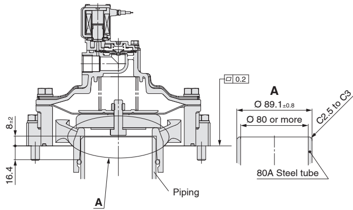
VXF26C□□□□ Piping
