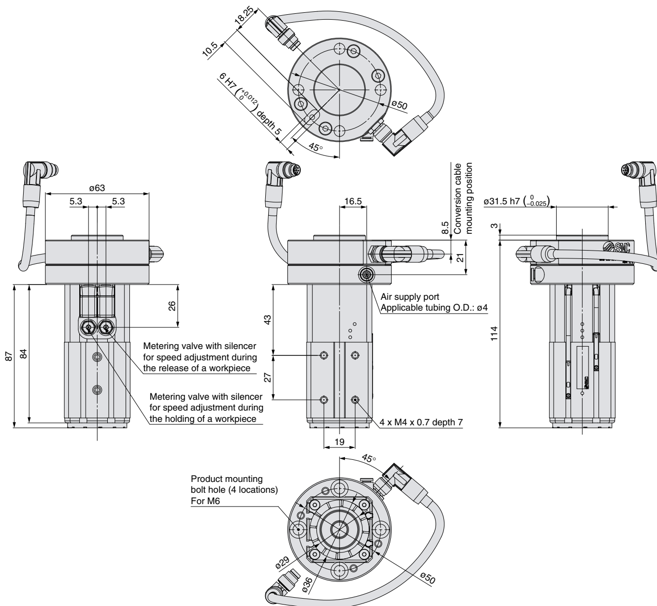
Magnet Gripper
