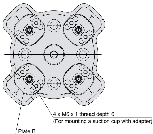
Suction cup with adapter mounting parts
