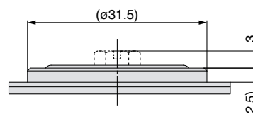
B (2:1) When the plug (M-5P) is mounted
