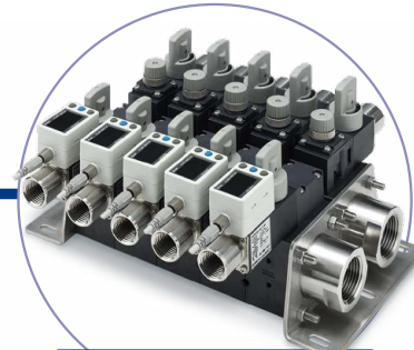
IO-Link Compatible Device: Digital Flow Switch for Water
