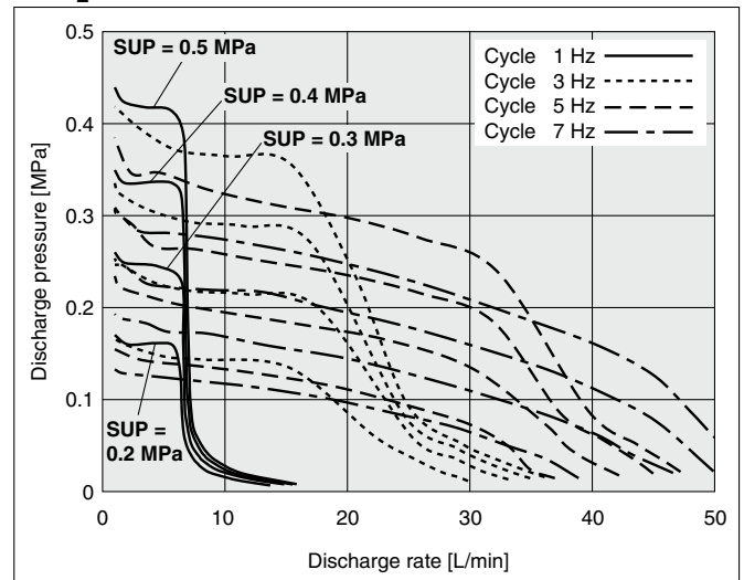
PA5 0 13 -□06 Flow Rate Characteristics
