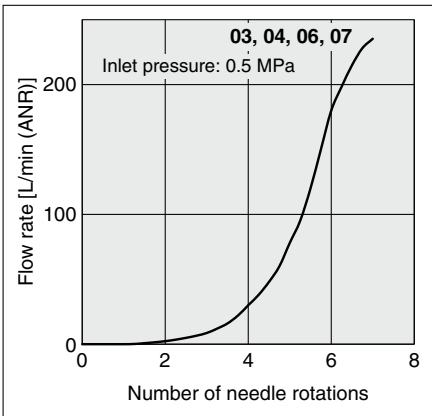
JASV-LE□□-□01 OUT-EXH. Flow rate
