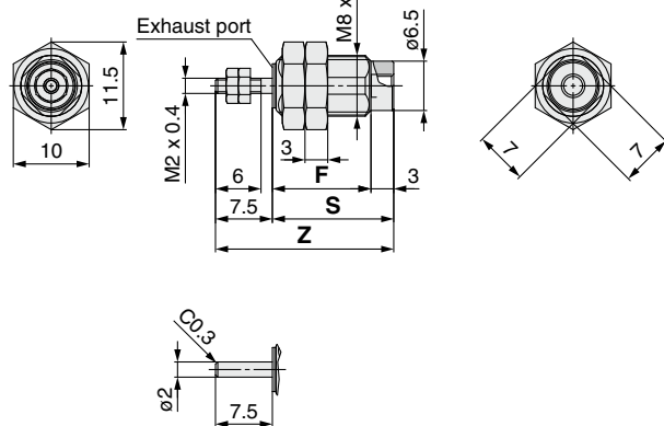
Without rod end thread CJPB4-□-B
