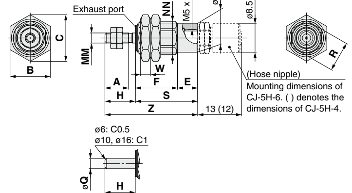
Without rod end thread CJPB□-□-B
