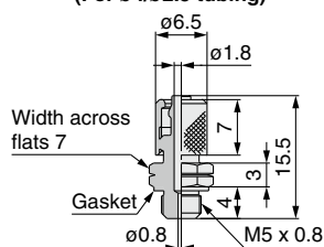
CJ-5H-4 (For ø4/ø2.5 tubing)
