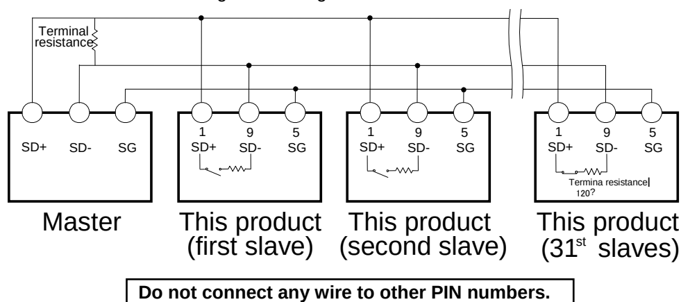
Fig 3.2-1 RS-485 connector connection
