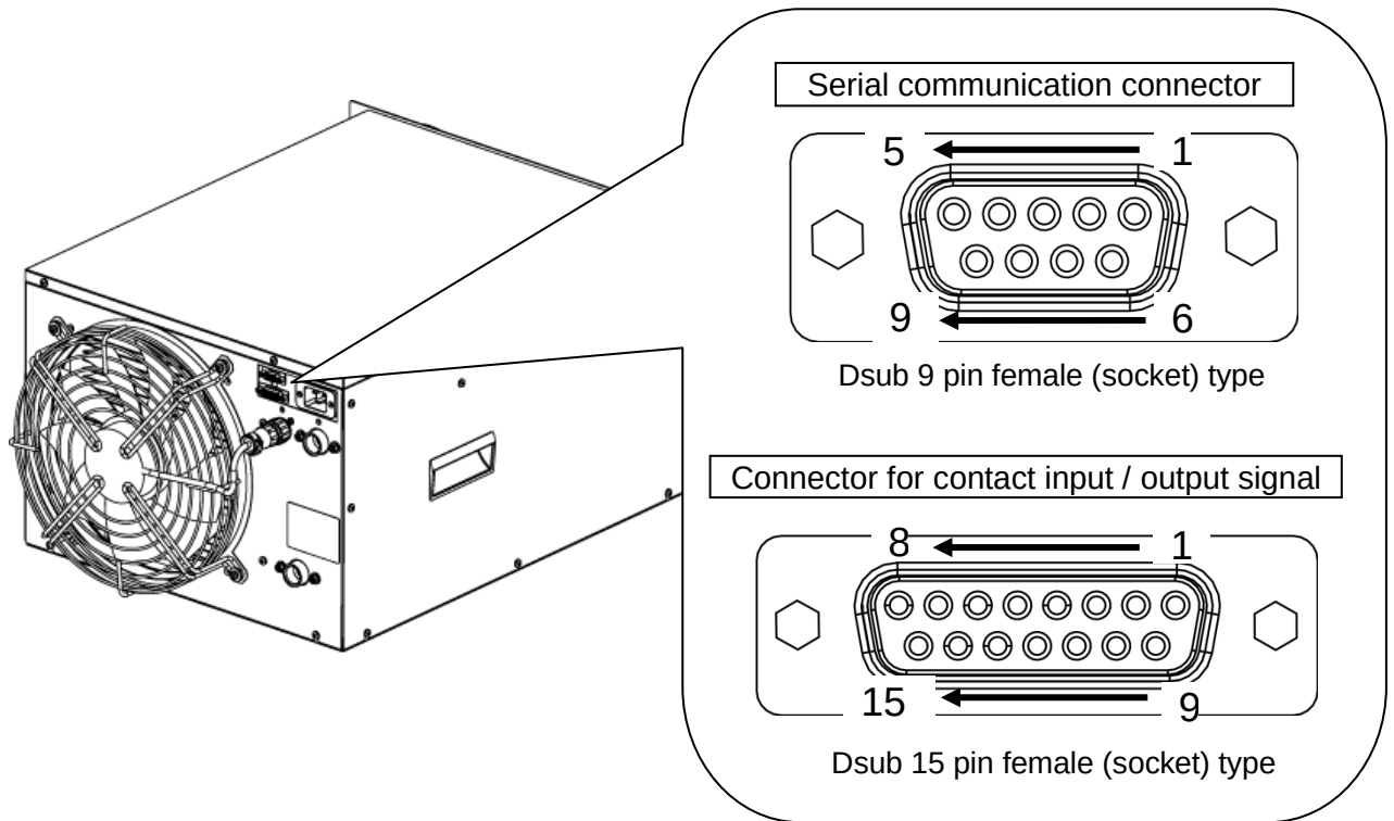
Fig 1.2-1 Communication port
